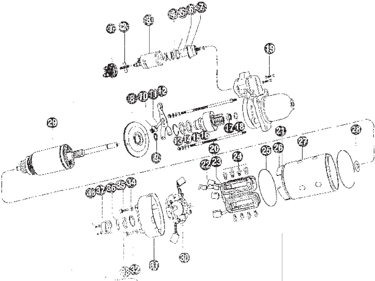
COMPONENT DETAIL OF STARTER MOTOR
