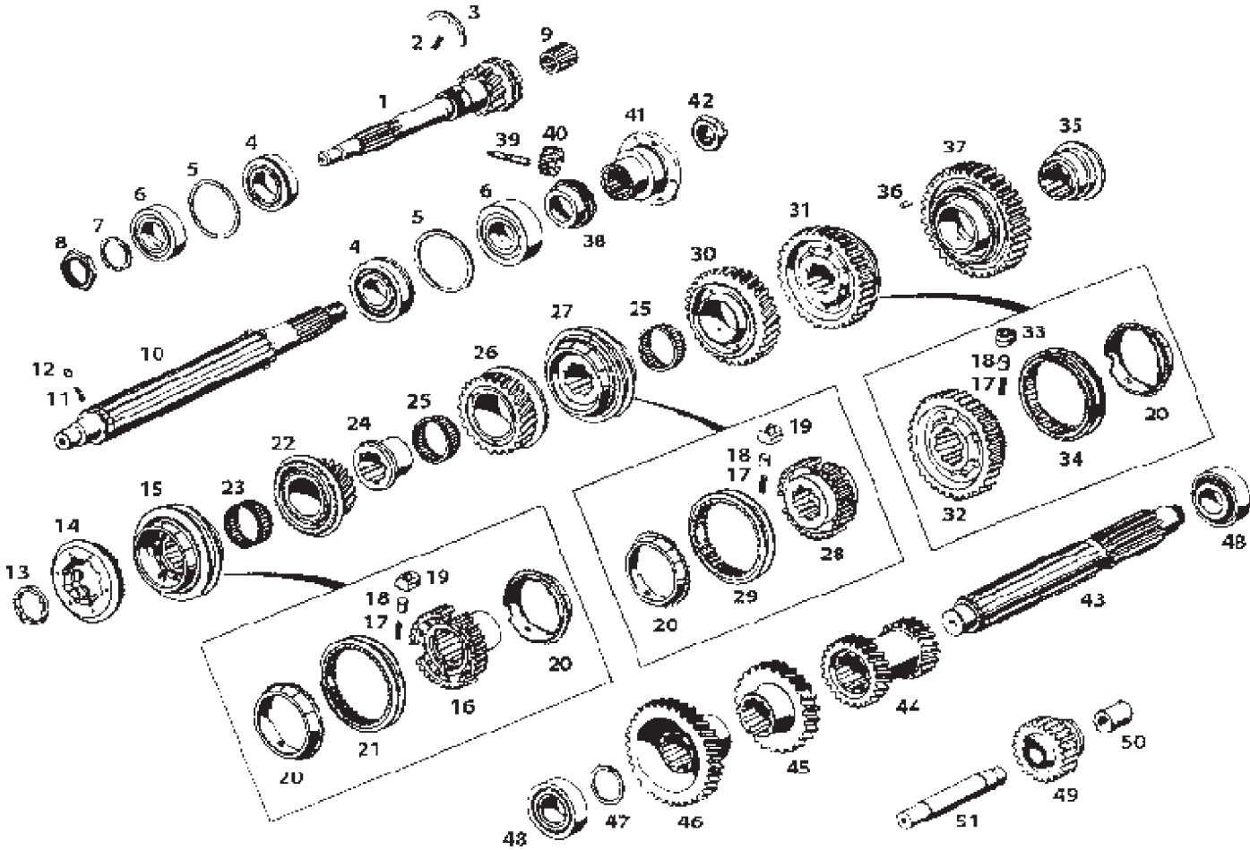
GEAR SHAFTS AND GEARS
