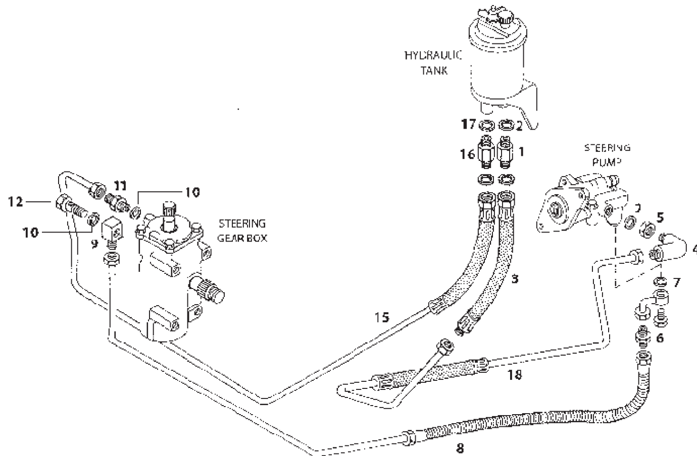
HYDRAULIC LINES (POWER STEERING)
