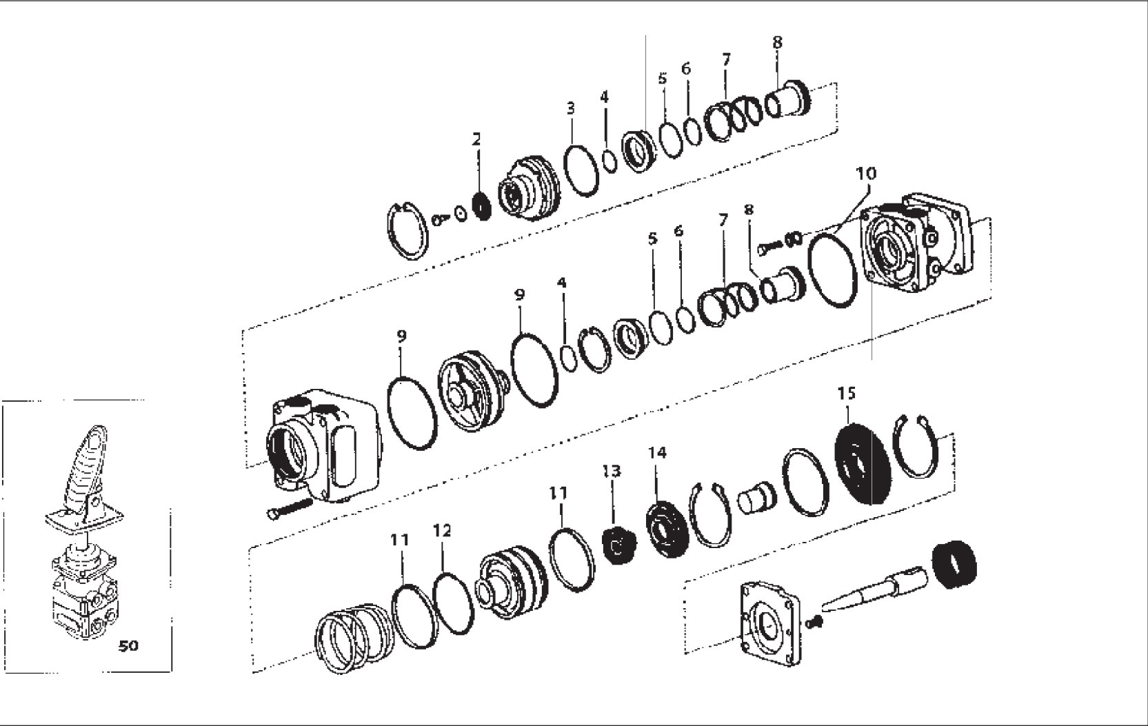
DUAL BRAKE VALVE
