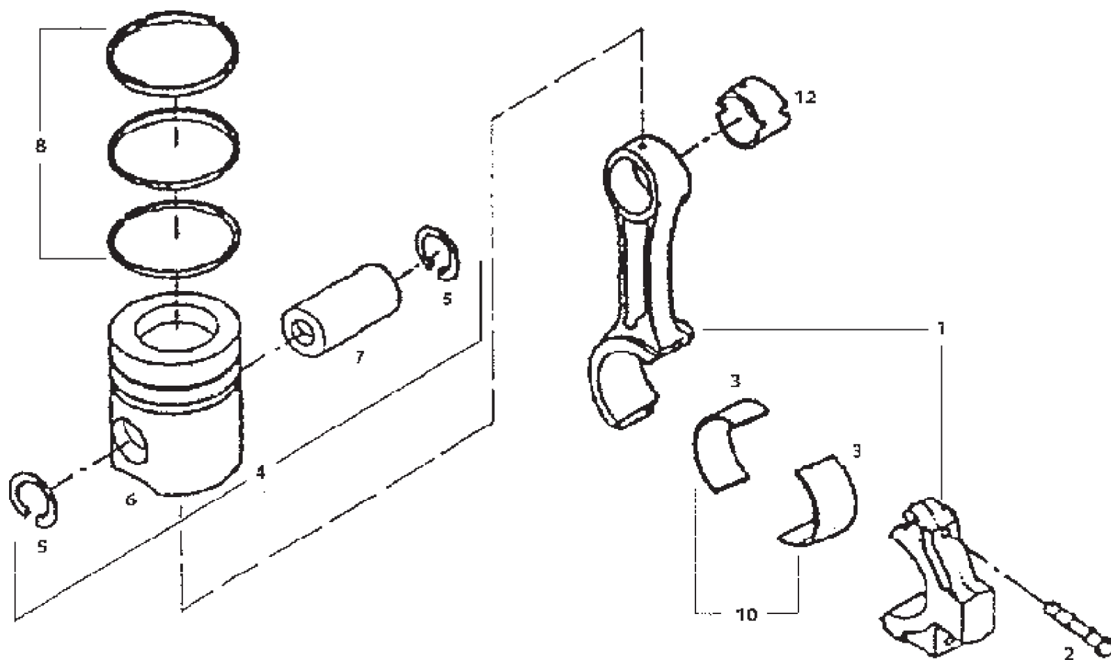
CONNECTING ROD AND PISTON
