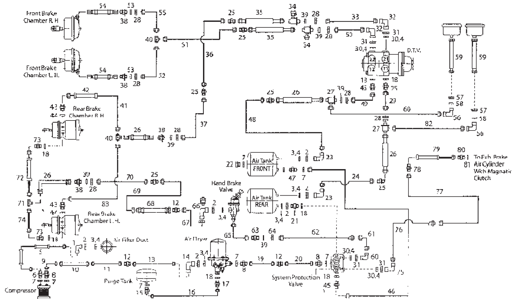
BRAKE PIPE LINES
