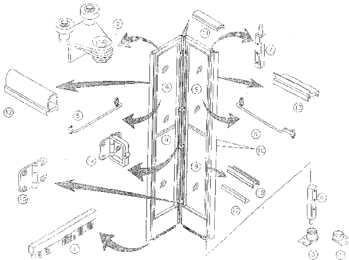
PASSENGER DOOR - JK TYPE
