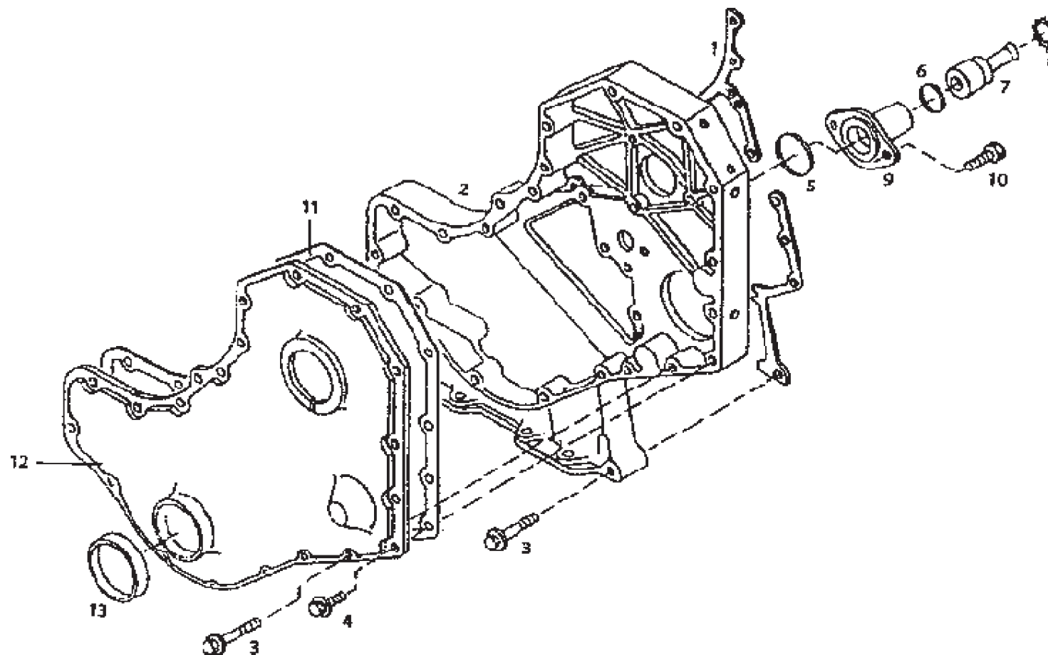
FRONT GEAR COVER
