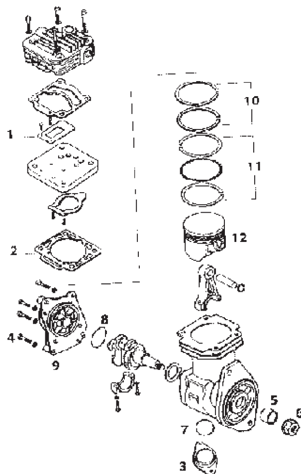
REPAIR KIT FOR AIR COMPRESSOR (NEW VERSION)
