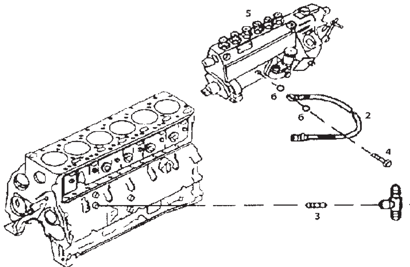
FUEL PUMP BASE
