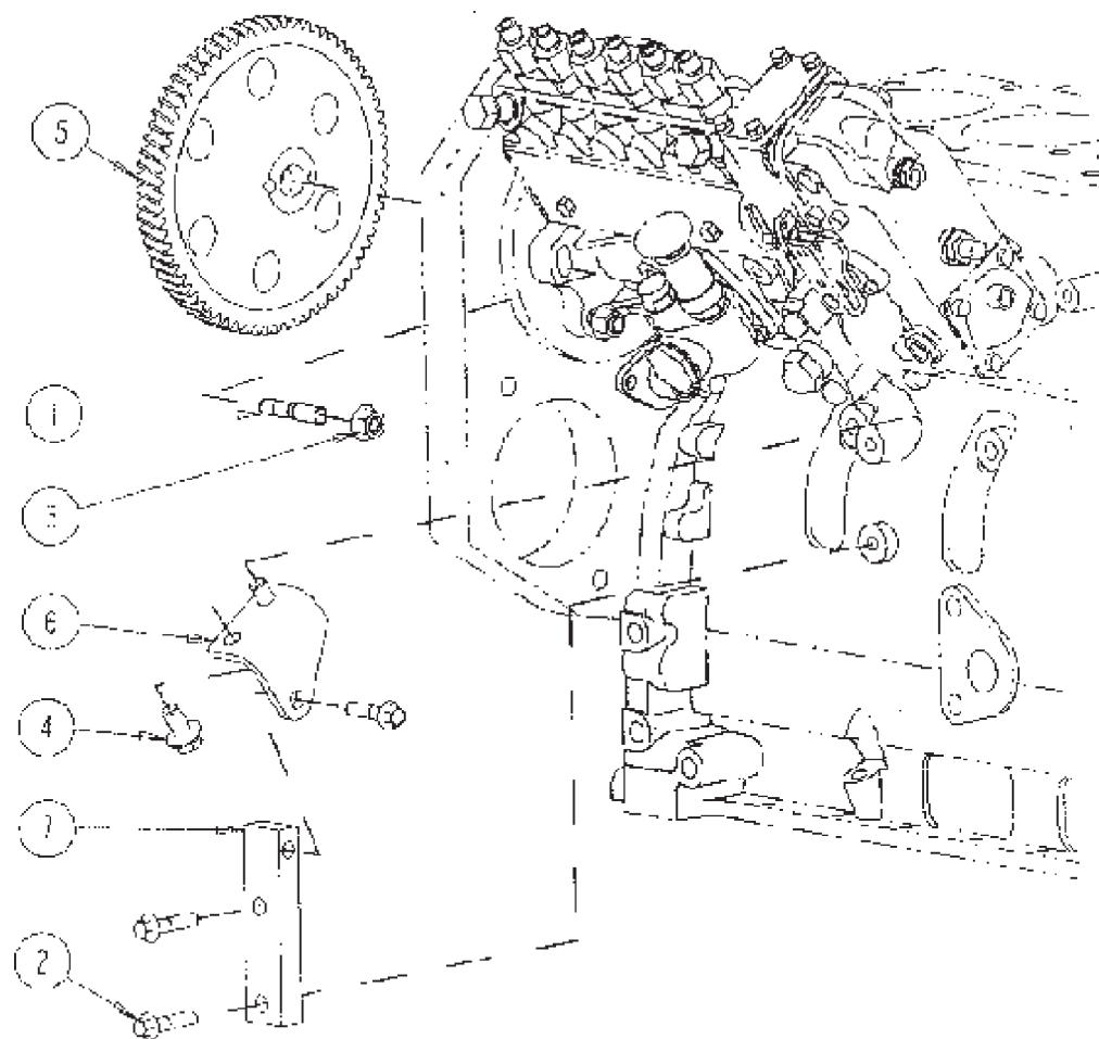
FUEL PUMP COUPLING
