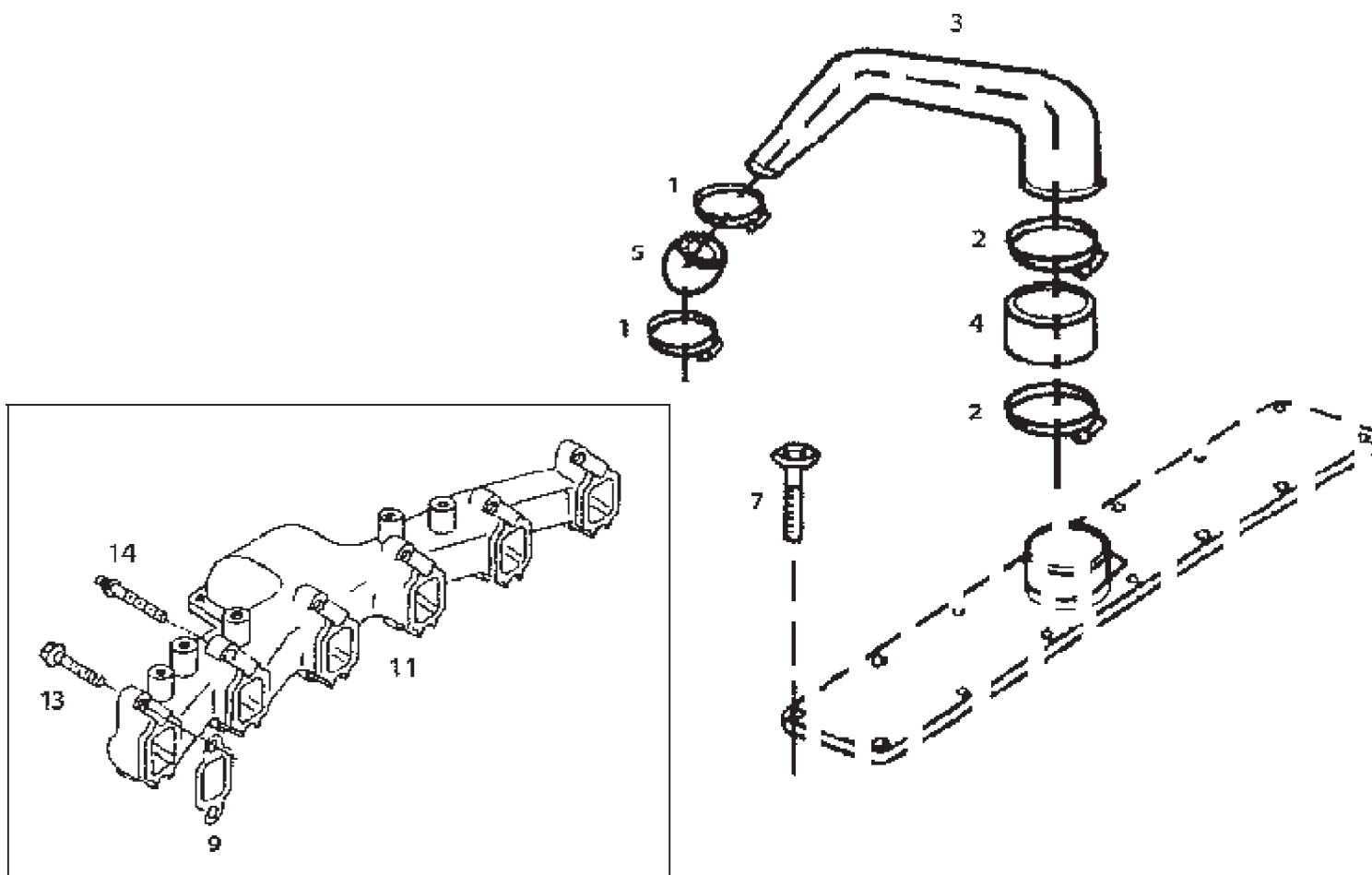
TURBOCHARGER LOCATION (LOW MOUNT)
