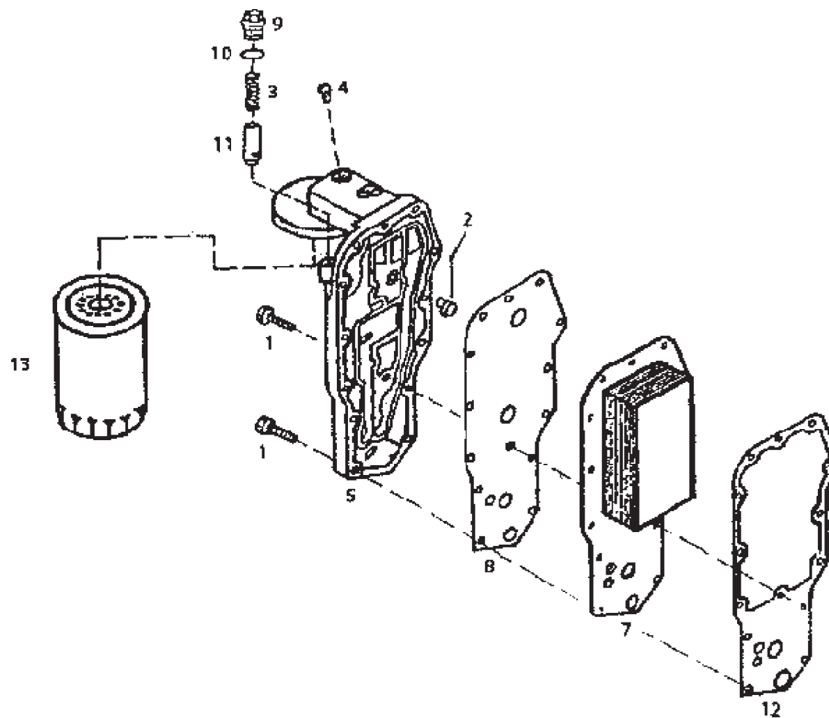
LUBRICATING OIL COOLING / OIL FILTER
