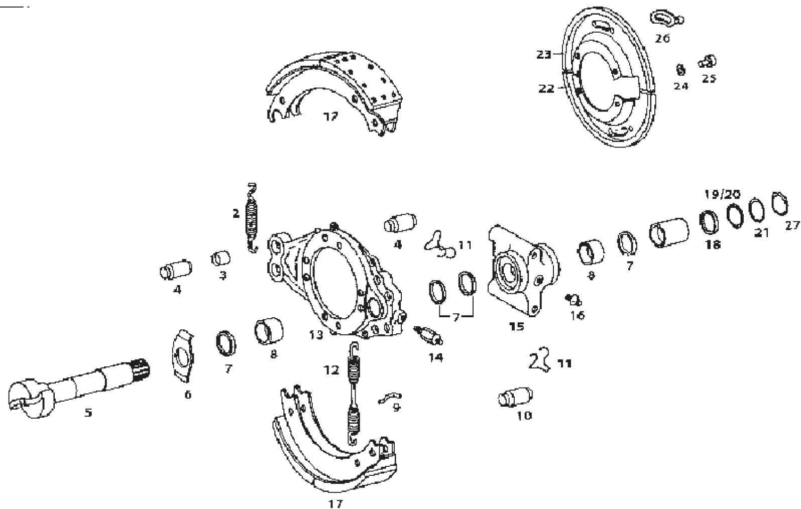
REAR WHEEL BRAKE (S-CAM) M/S. AAL
