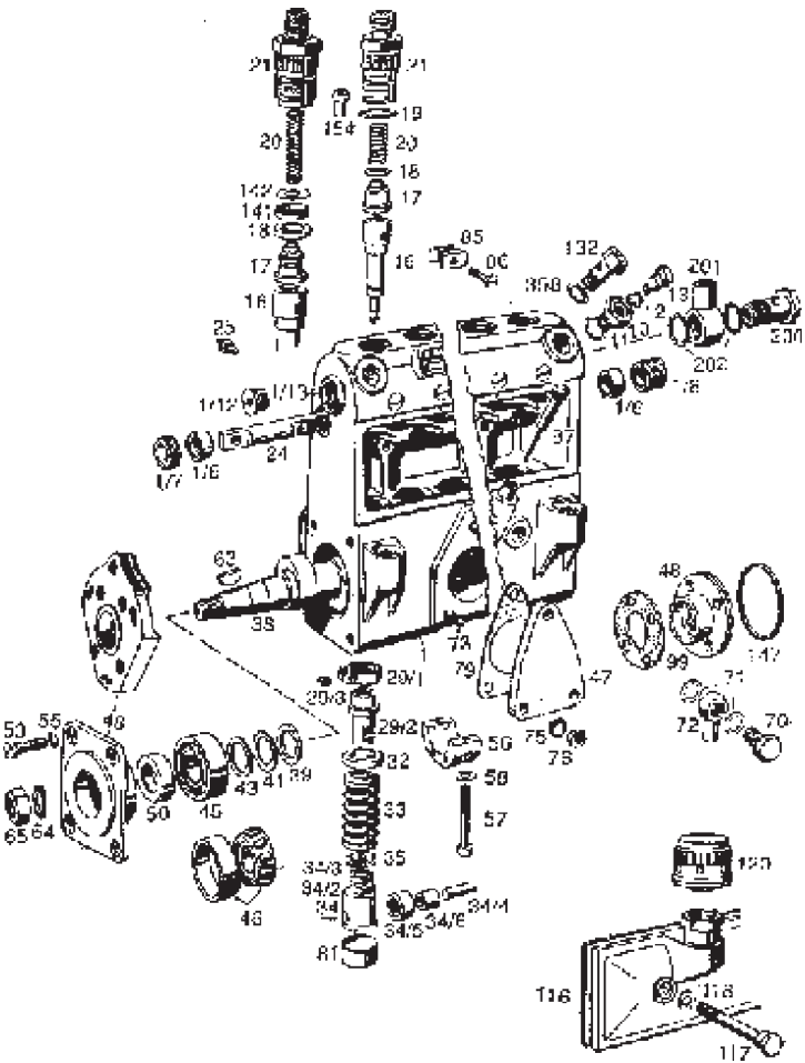
FUEL INJECTION PUMP
