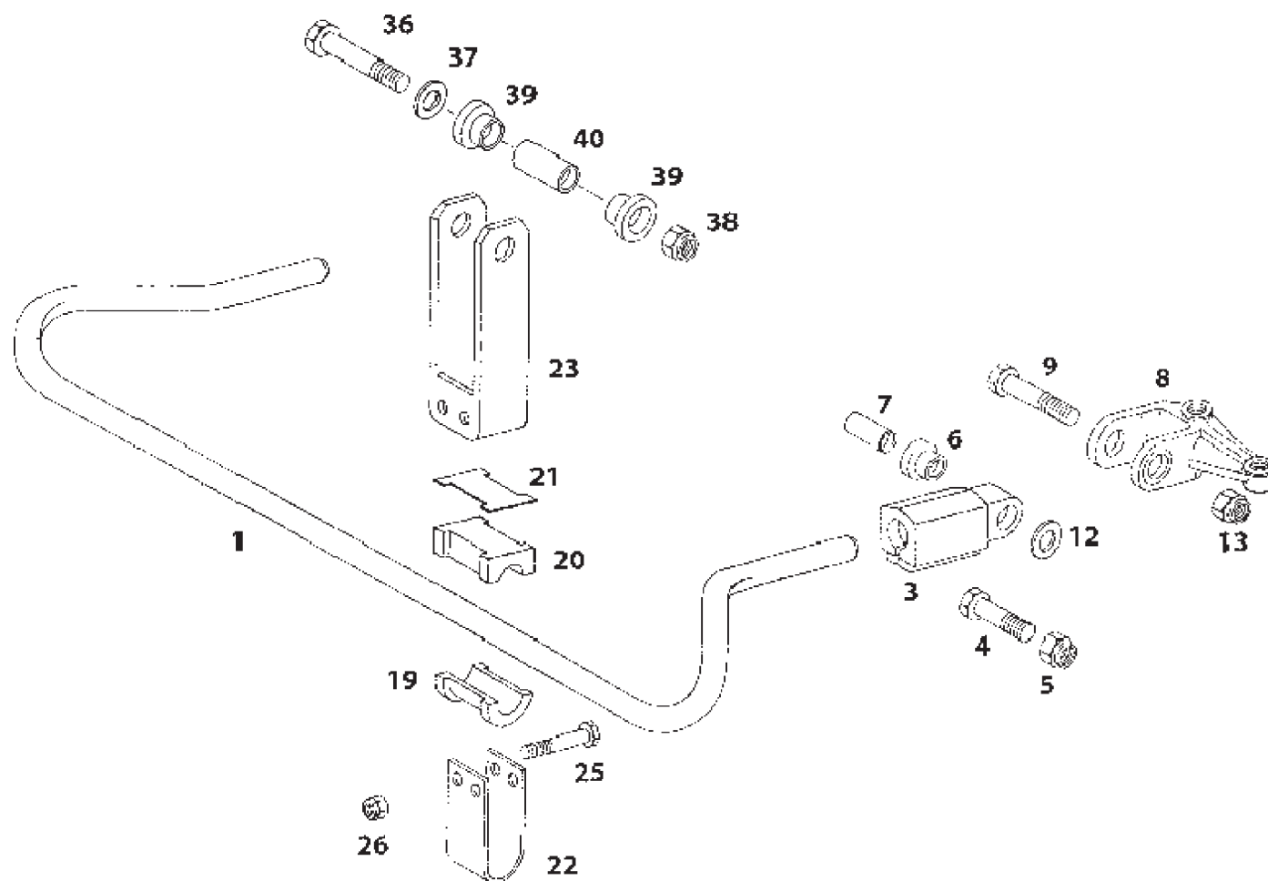
FRONT ANTI-ROLL BAR
