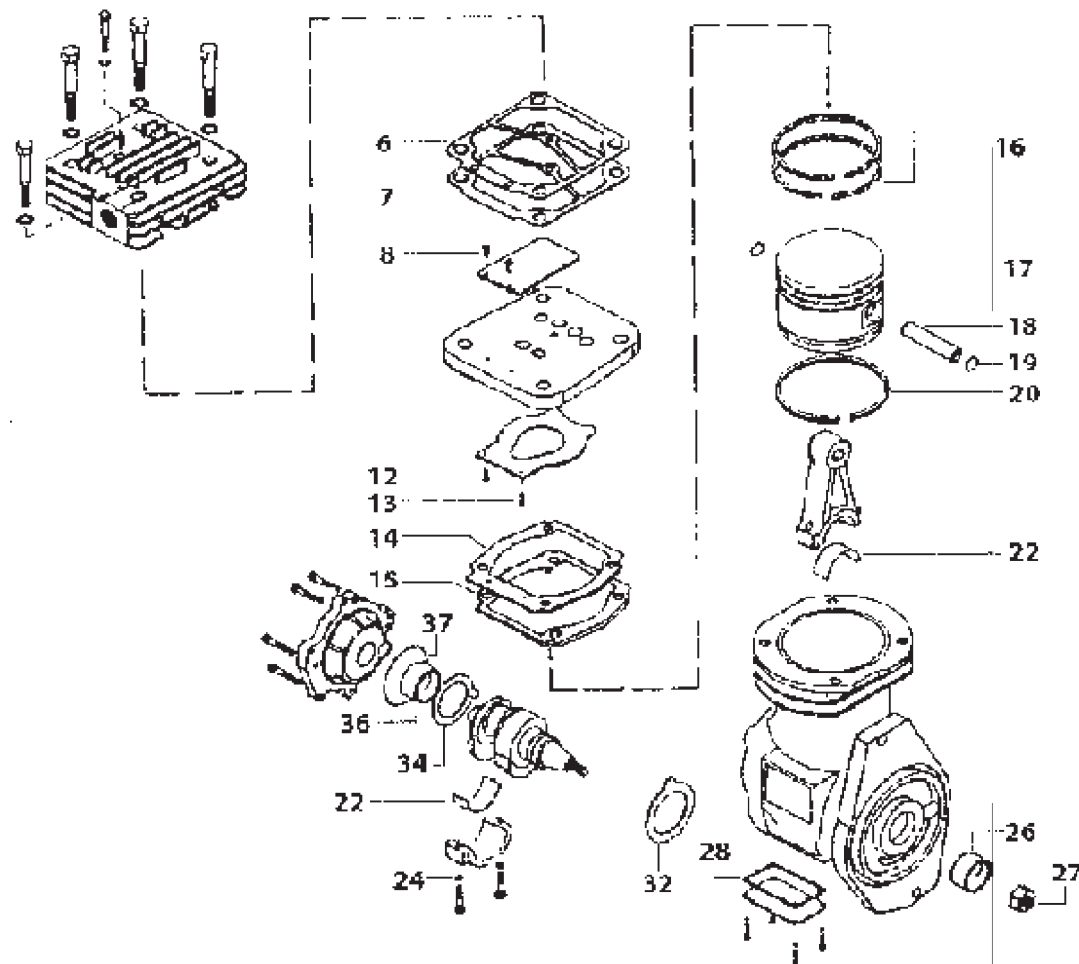
REPAIR KIT FOR AIR COMPRESSOR
