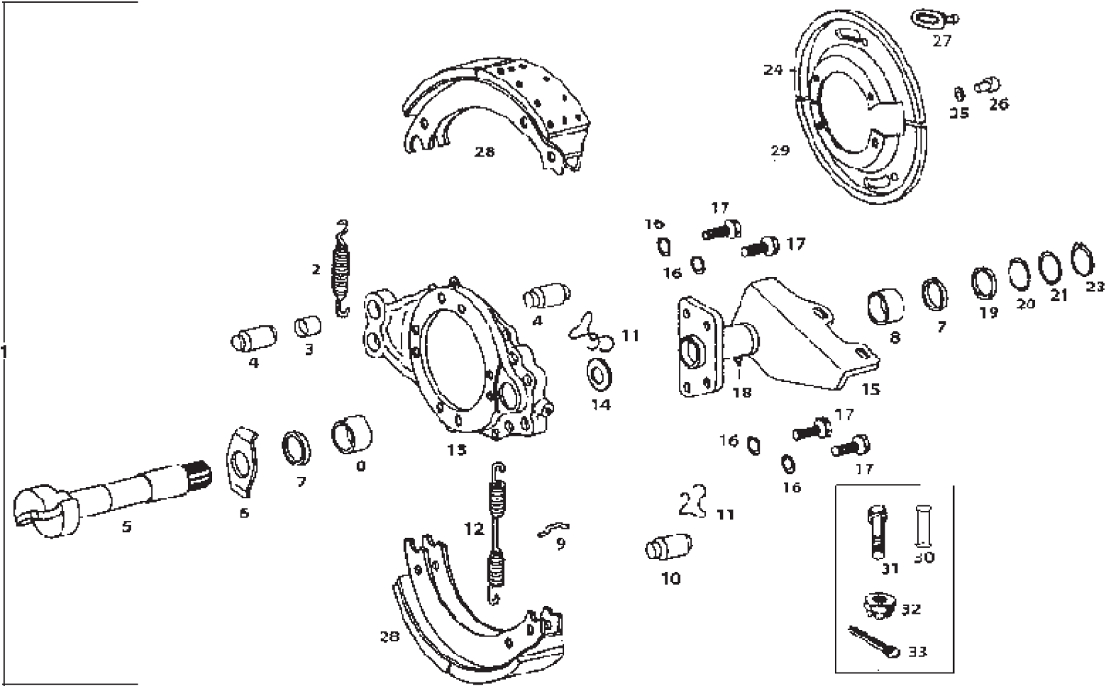
FRONT WHEEL BRAKE (S-CAM) (AAL)
