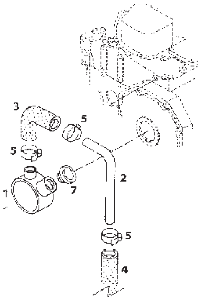
OIL FILL LOCATION
