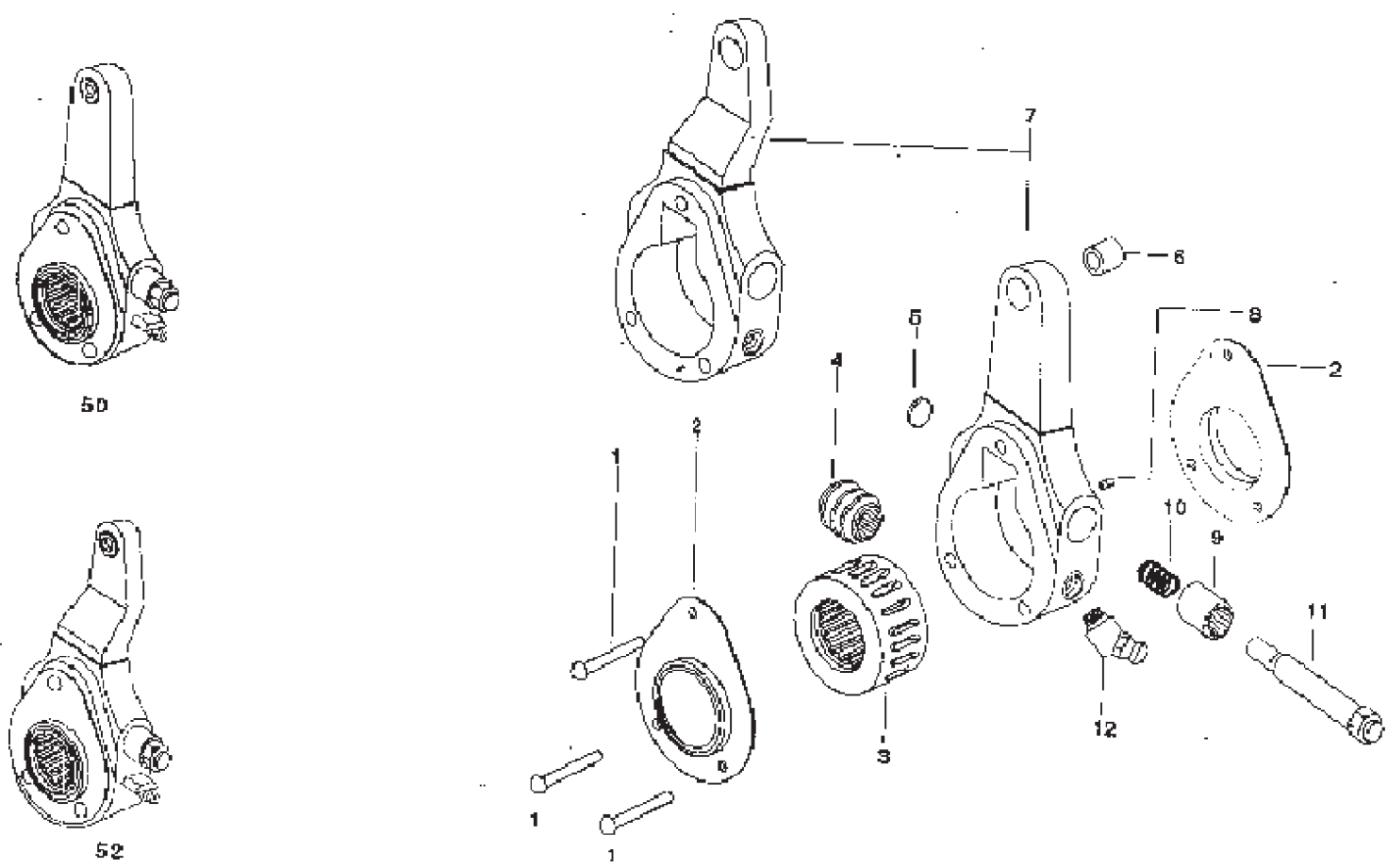
SLACK ADJUSTER (FRONT & REAR)
